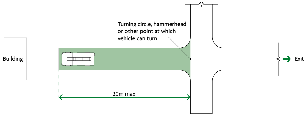
Diagram 15.3 Turning facilities
